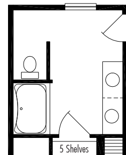
Master Bath Option GHB2 Garden Tub in Place of 5' Shower Unit
