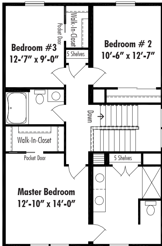
Grafton Hill I A 25' x 38' Second Floor
