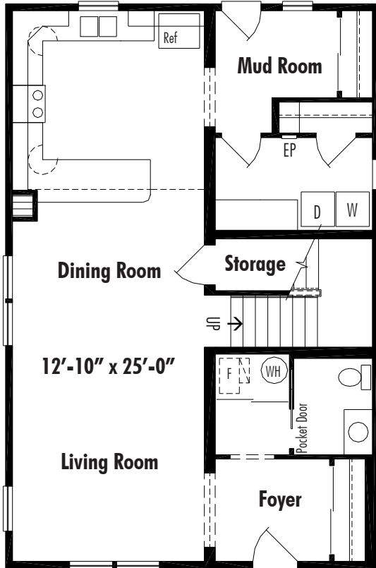
Grafton Hill I A Crawl Space 25' x 38' 1900 Sq. Ft. Total Living Area
