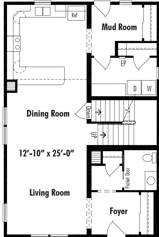
Grafton Hill I B Basement 25' x 38' 1900 Sq. Ft. Total Living Area
